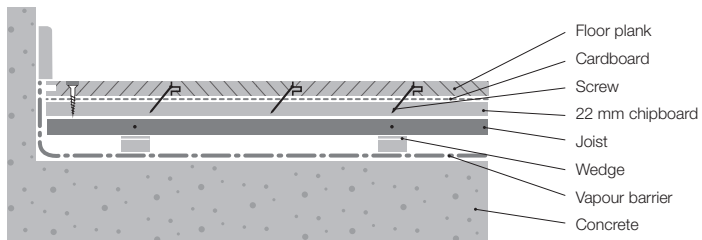
Figure 8: Cross section, secretly screwed, joists
