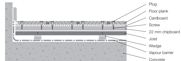
Figure 7: Cross section, screwed from above, joists
