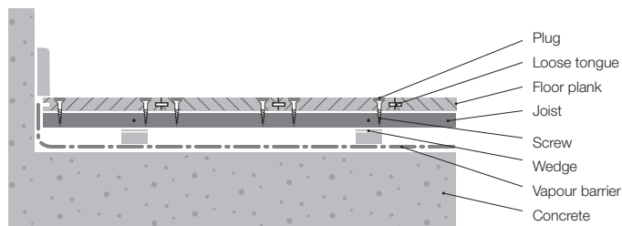
Figure 3: Cross section, screwed from above, joists
