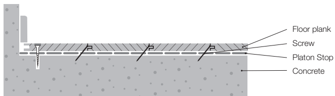
Figure 5: Cross section, secretly screwed
